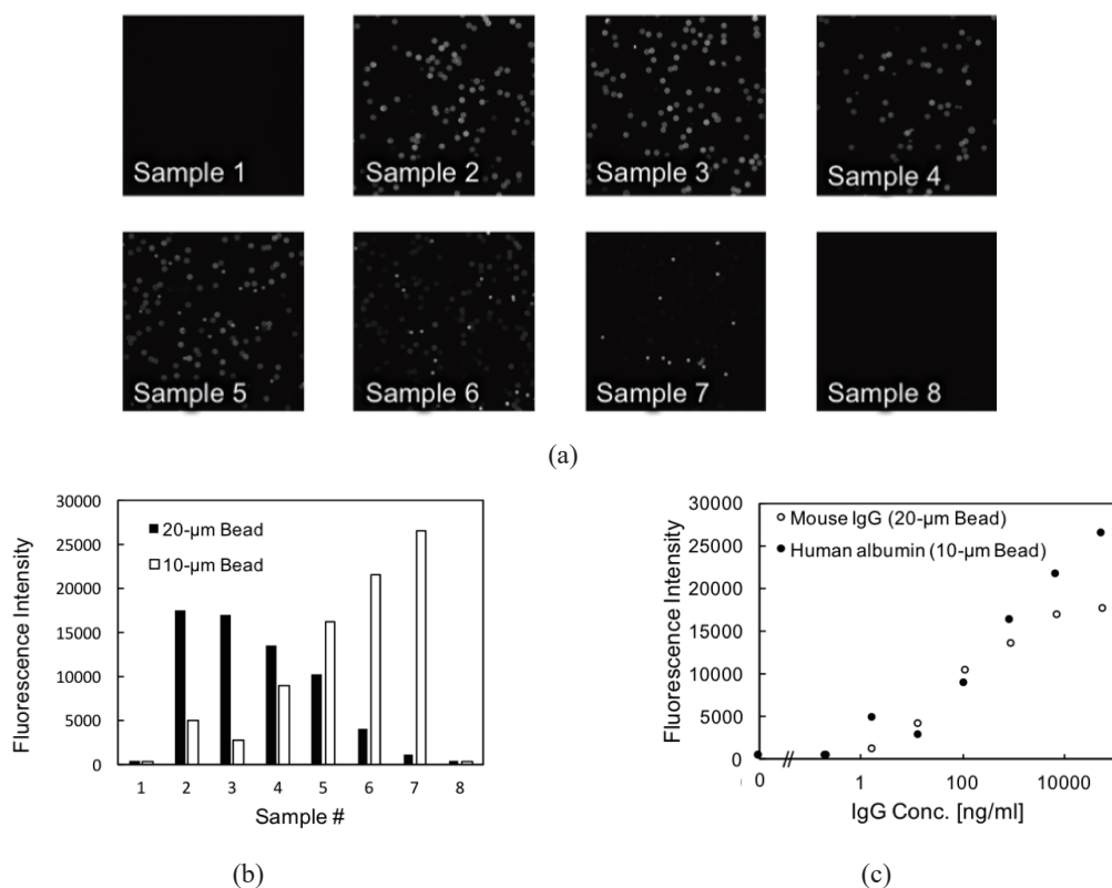
Fig. 3. (a) Fluorescence image of microbeads after immunoreactions. (b) Immunoreaction of the anti-human albumin antibody-immobilized microbeads (10 \mu\text{m} ) and the anti-mouse IgG antibody-immobilized microbeads (20 \mu\text{m} ) with a mixture of mouse IgG and human albumin at various concentrations. (c) Calibration curves plotting the relationship between fluorescence of the 10 \mu\text{m} microbeads and the concentration of human albumin, and fluorescence of 20 \mu\text{m} microbeads and the concentration of mouse IgG.
